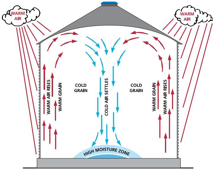
WITHOUT AN AERATION SYSTEM
